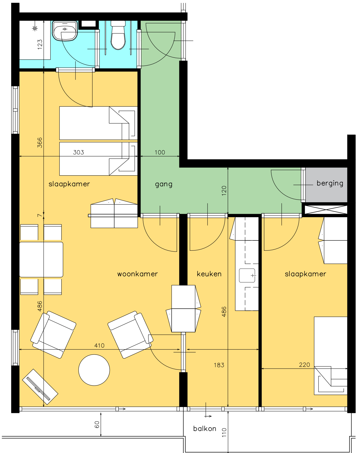
Serviceflat "Seine" – type A
